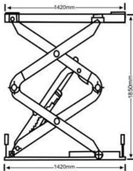
OVERALL STRUCTURE SIZE (mm)
